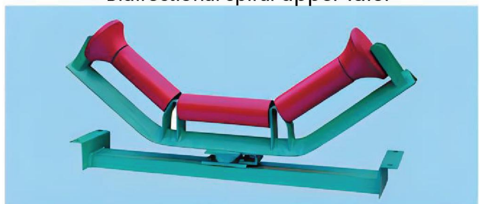
Friction self-aligning upper idler
