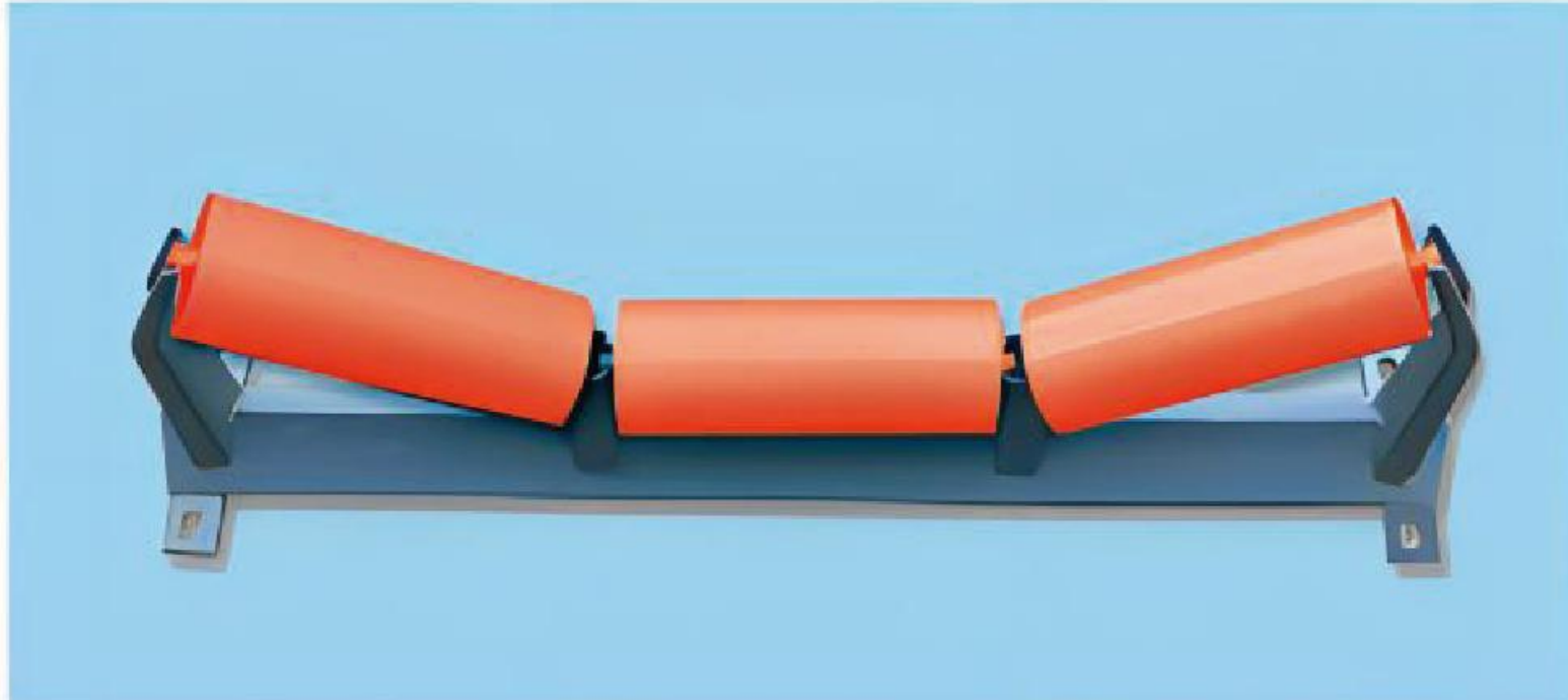
Trough idler
